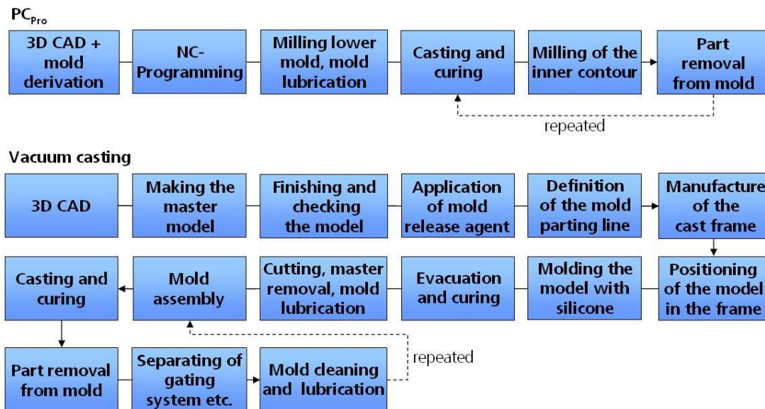
Figure 3: Comparison of RP process chains
